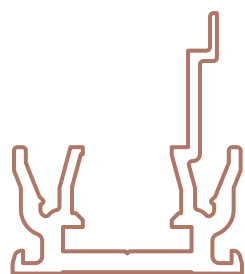
PROFILO BASE VERTICALE MAIN PROFILE 16.156
